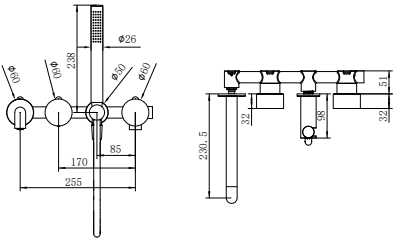
NR252003b230 Opal Progressive Shower System Separate Plate With Spout 230mm Wels Rating: 7.5L/Min, Not Star Rated Material: Brass
